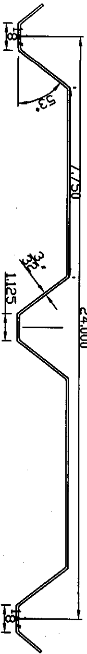
ALTERNATE "B" 12" CORRUGATED PANEL (GE LEXAN 103/BAYER MAKROLON 3103/POLYONE/SPARTECH) Fu = 9367 PSI, Fy = 91346 PSI SCALE: 3" = 1'-0"
