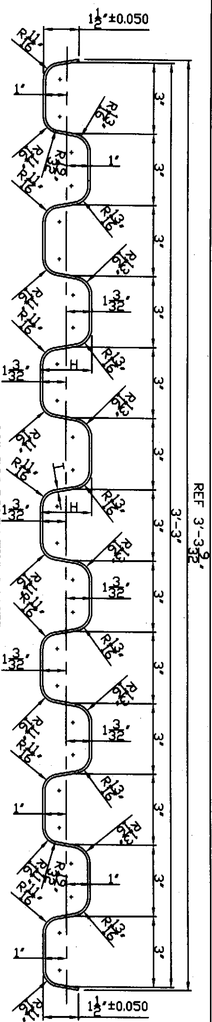
39" CORRUGATED PANEL (GE LEXAN 103/BAYER MAKROLON 3103/POLYONE/SPARTECH) Fu = 9367 PSI, Fy = 91346 PSI SCALE: 3" = 1'-0"
